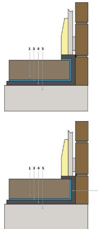
Perimeter Details
